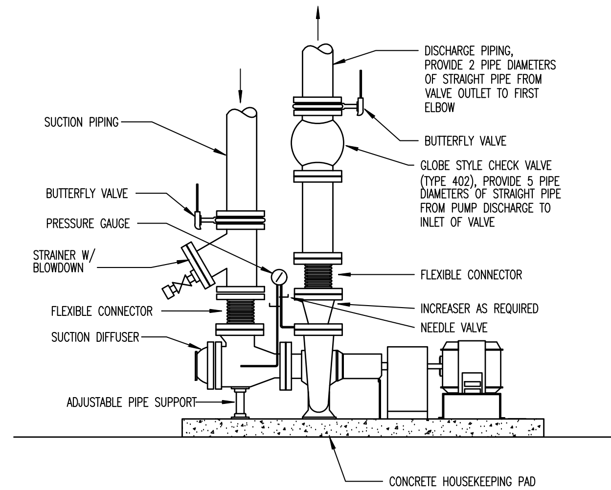
3 - BASE MOUNTED PUMP DETAIL SCALE: NTS
