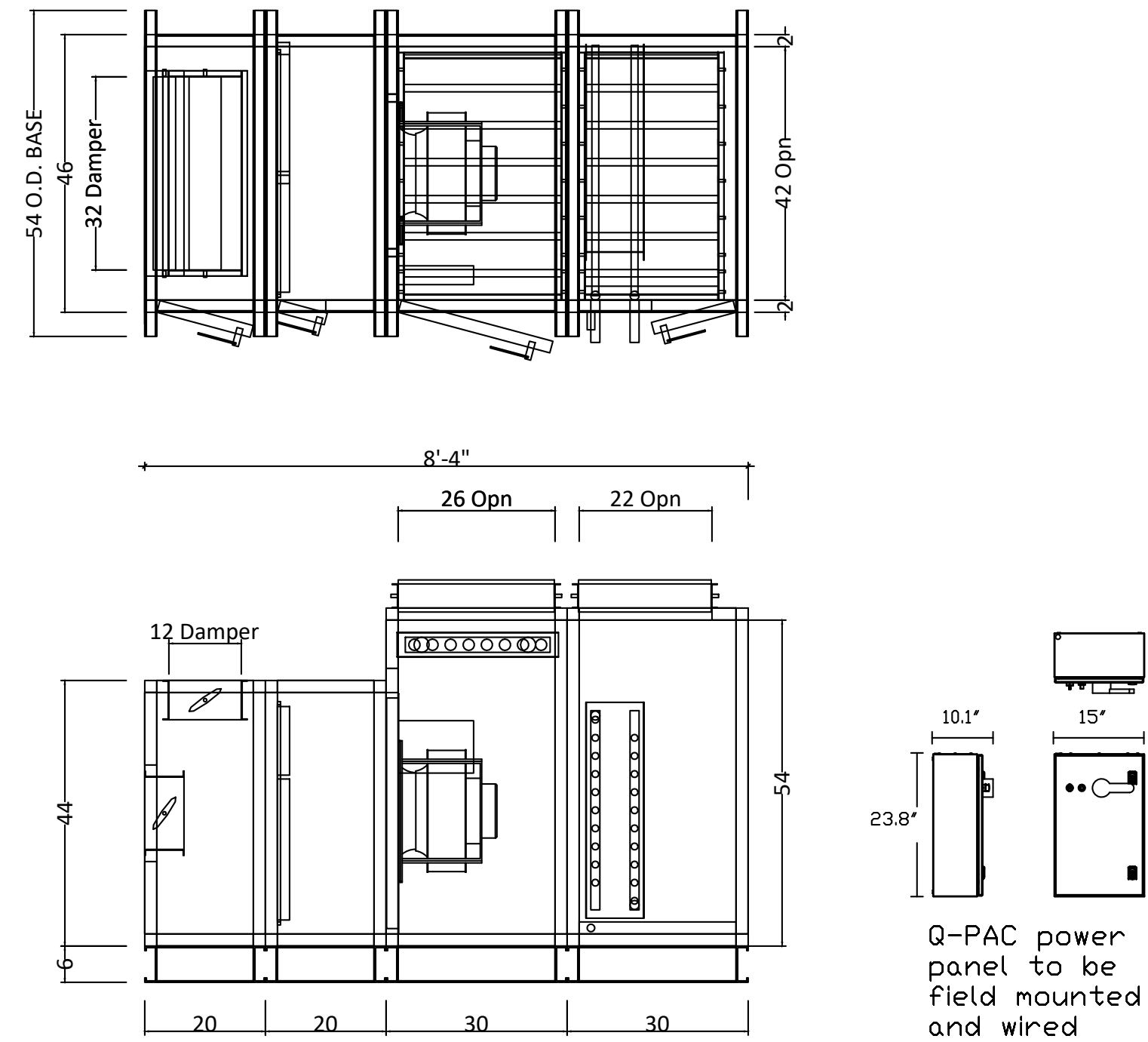
4 - AHU-8 DIMENSIONAL DRAWING
